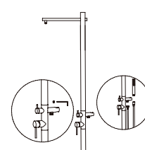
Step 5.Connect the faucet body with the pipes
