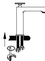
Step 3. Install screw stick to faucet body
