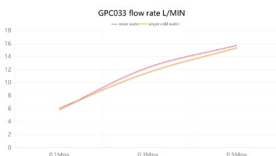
shower head
